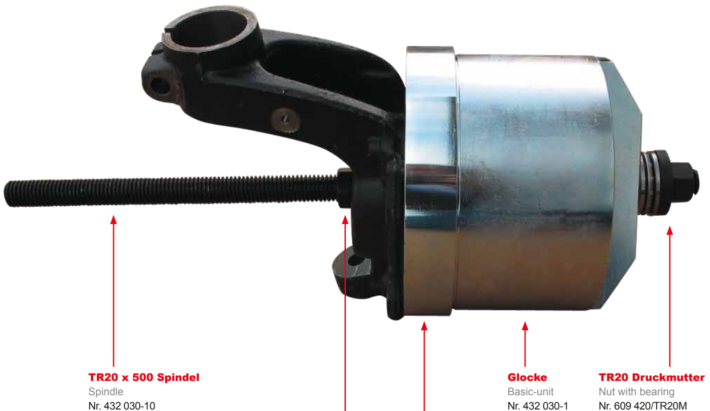
3-Punkt Auszieh-Adapterring 3-point adapter-ring Nr. 432 030-6
